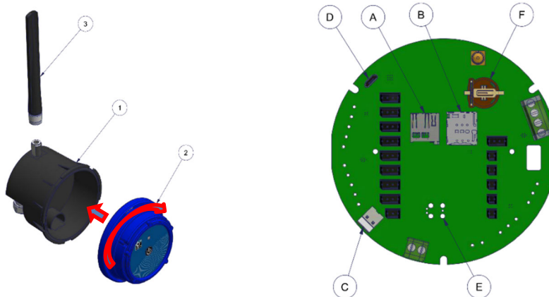
Figure 3 Body (1) and head (2) assembly
